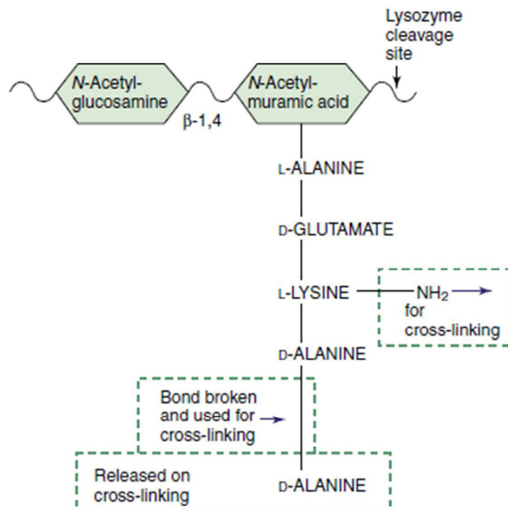
Fig. 12.6 Precursor of peptidoglycan. The peptidoglycan is built from prefabricated units that contain a pentapeptide attached to the N -acetylmuramic acid. The pentapeptide contains a terminal D-alanine-D-alanine unit. This dipeptide is required for cross-linking the peptidoglycan and is the basis for the action of \beta -lactam and vancomycin antibiotics. The \beta -1,4 disaccharide link cleaved by lysozyme is indicated.
