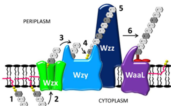
Fig. 1. Schematic of the Wzx/Wzy-dependent assembly pathway. 1. Polysaccharide repeat units are built in the cytoplasm by a series of glycosyltransferase proteins on the lipid carrier UndPP, resulting in the sugar repeat linked to UndPP. 2. UndPP-linked repeat units are flipped from the cytoplasmic leaflet to the periplasmic leaflet of the IM by Wzx. 3. The flipped UndPP-linked repeat units are obtained by Wzy. 4. Wzy-mediated polymerization of the repeat units is carried out at the reducing terminus of the growing chain. 5. The length of polymerization is governed by the chain length regulator Wzz, resulting in preferred modal lengths of polymer. 6. For LPS, the polymerized glycan is ligated to lipid A-core oligosaccharide by WaaL to form a mature LPS molecule.
